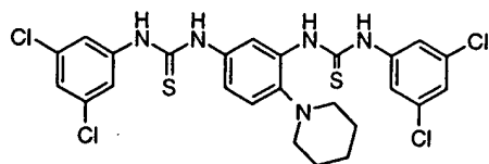
Compound # 44
